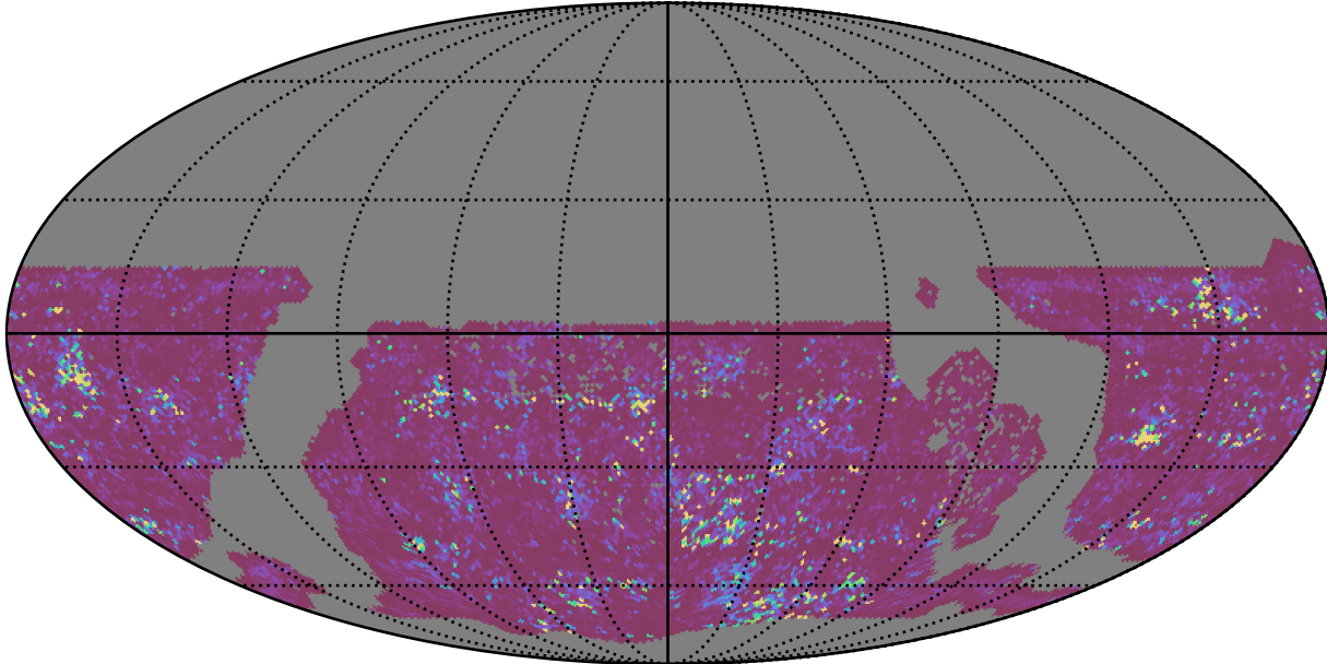
too_elab_r32_d2_giz_v3.4_10yrs WFD g band: 75th Percentile Intranight Timespan
