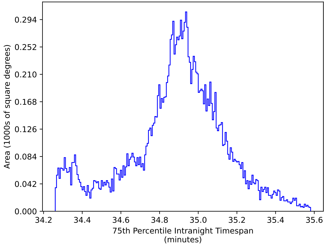
too_elab_r32_d2_giz_v3.4_10yrs WFD all bands: 75th Percentile Intranight Timespan
