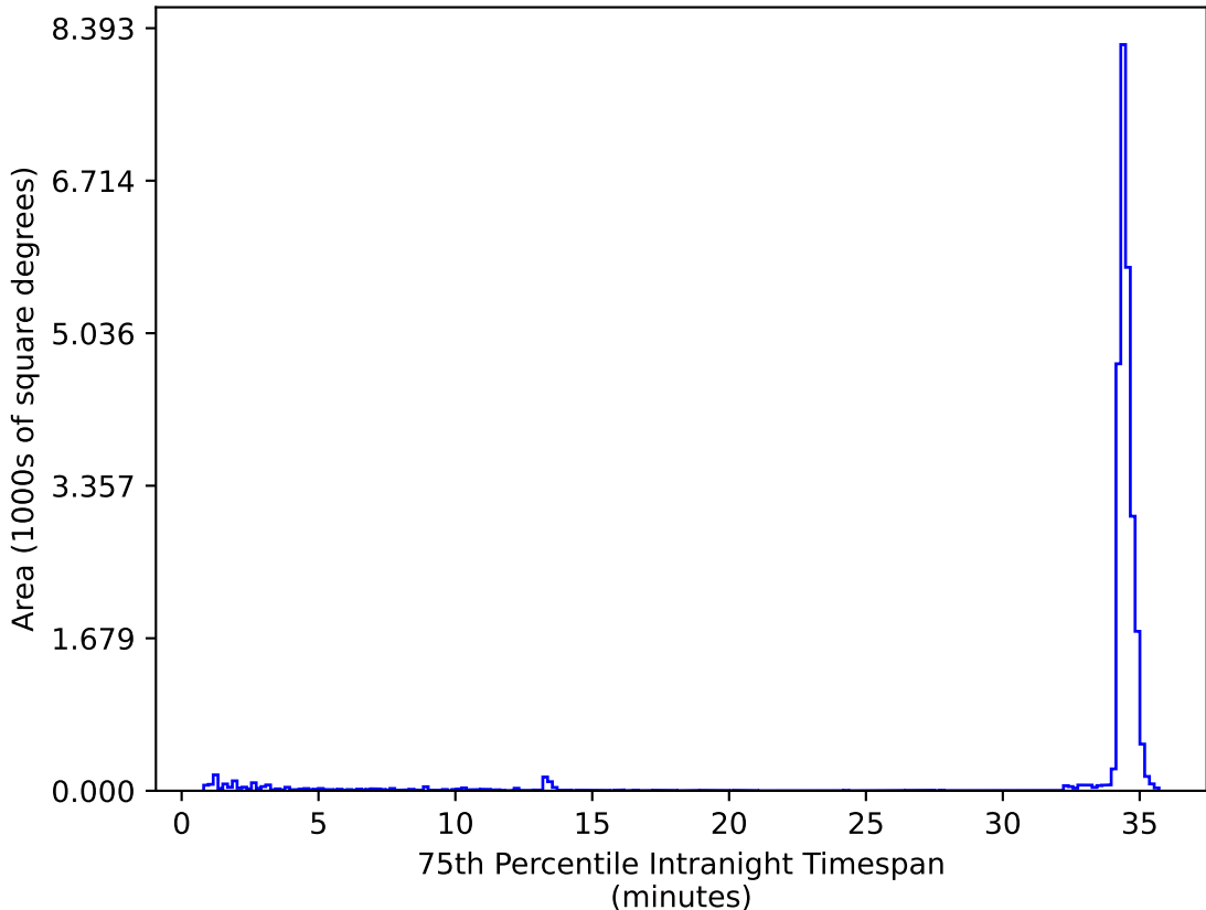
too_elab_r32_d2_giz_v3.4_10yrs All sky zy bands: 75th Percentile Intranight Timespan
