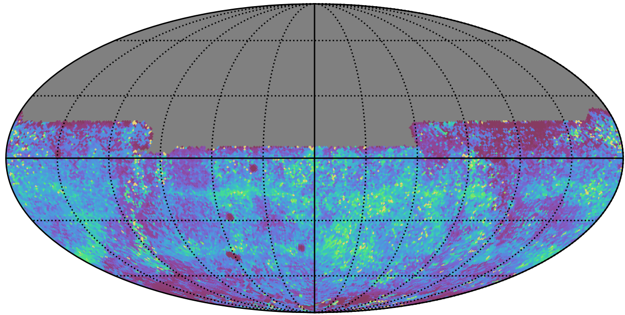
too_elab_r32_d2_giz_v3.4_10yrs All sky y band: 75th Percentile Intranight Timespan
