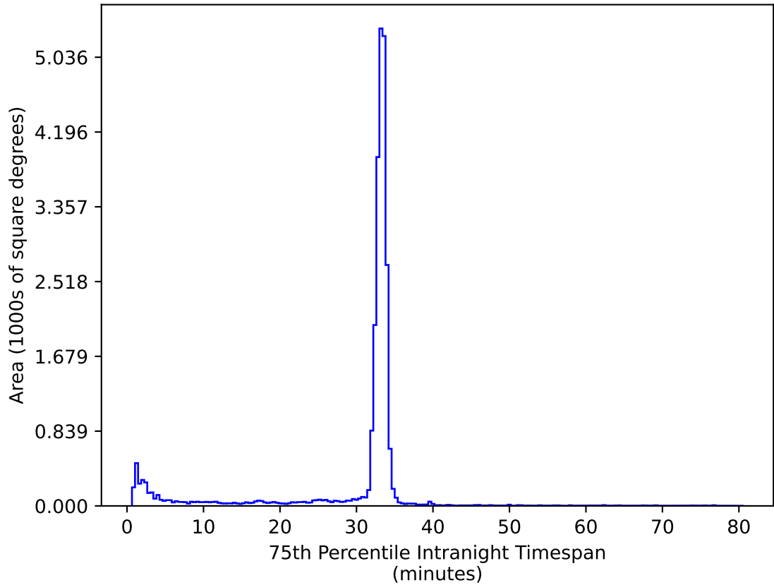
too_elab_r32_d2_giz_v3.4_10yrs All sky ug bands: 75th Percentile Intranight Timespan
