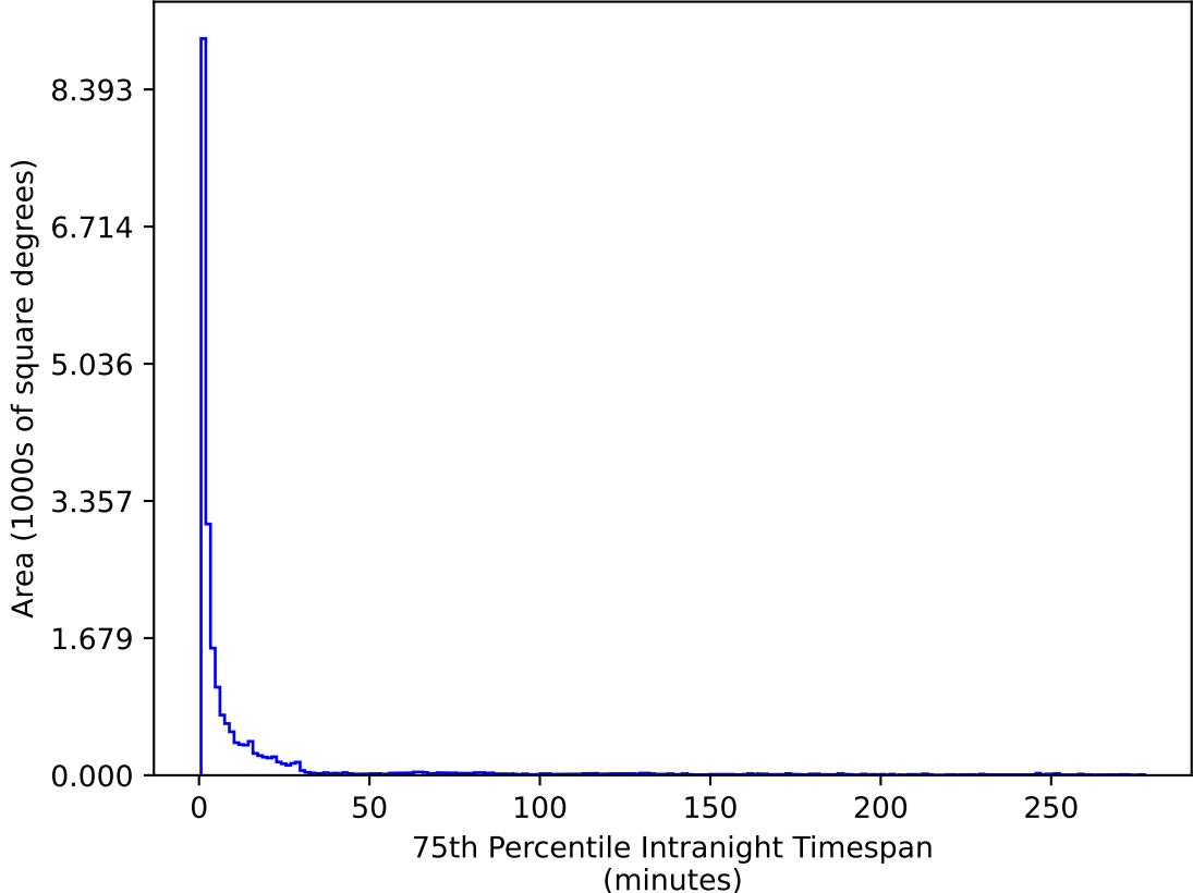
too_elab_r32_d2_giz_v3.4_10yrs All sky u band: 75th Percentile Intranight Timespan
