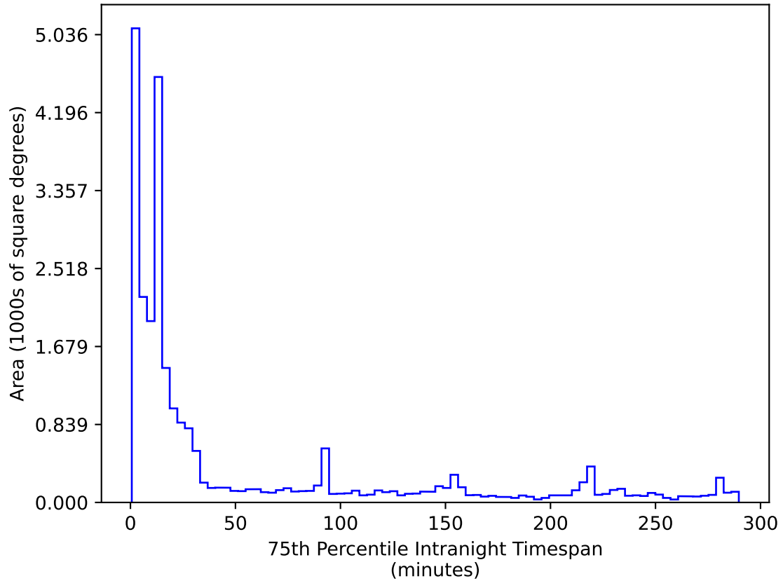
too_elab_r32_d2_giz_v3.4_10yrs All sky r band: 75th Percentile Intranight Timespan
