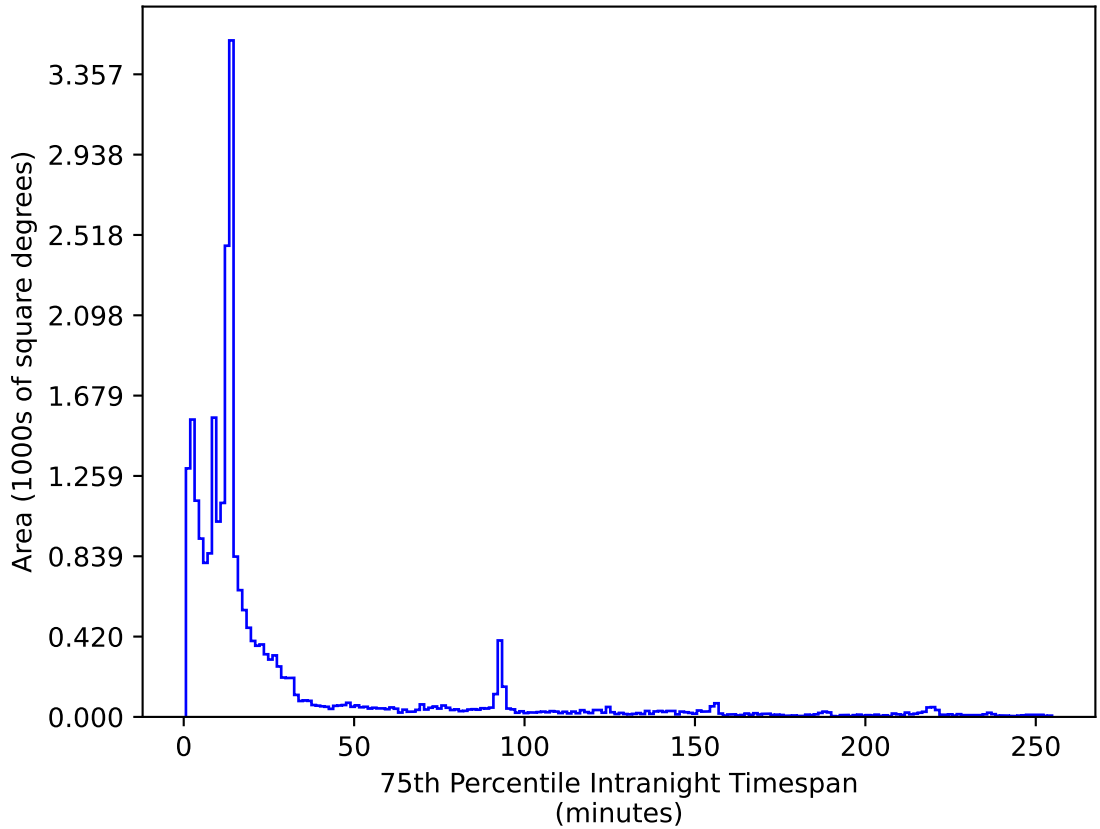
too_elab_r32_d2_giz_v3.4_10yrs All sky i band: 75th Percentile Intranight Timespan
