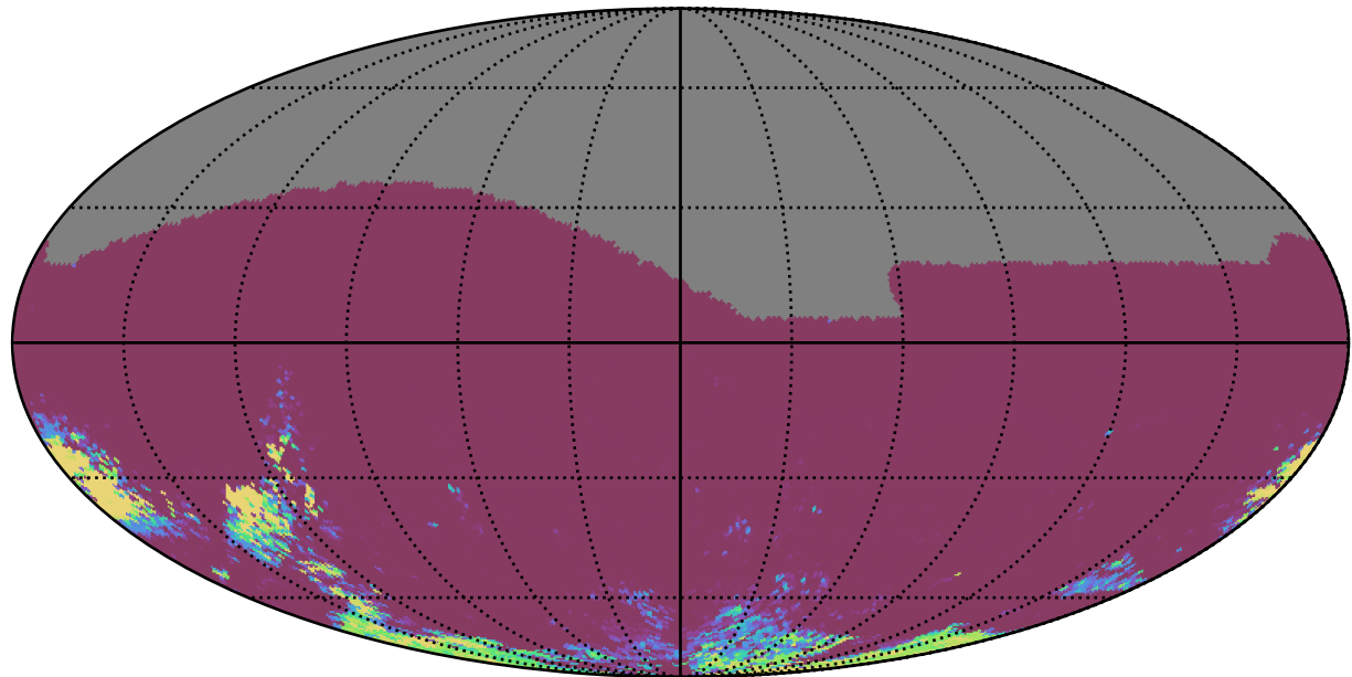
too_elab_r32_d2_giz_v3.4_10yrs All sky gr bands: 75th Percentile Intranight Timespan
