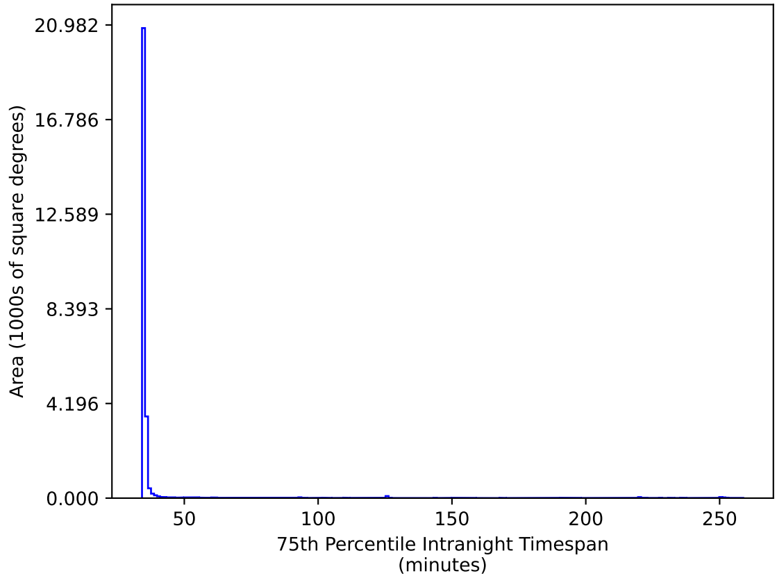
too_elab_r32_d2_giz_v3.4_10yrs All sky gr bands: 75th Percentile Intranight Timespan
