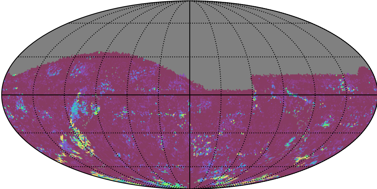
too_elab_r32_d2_giz_v3.4_10yrs All sky g band: 75th Percentile Intranight Timespan
