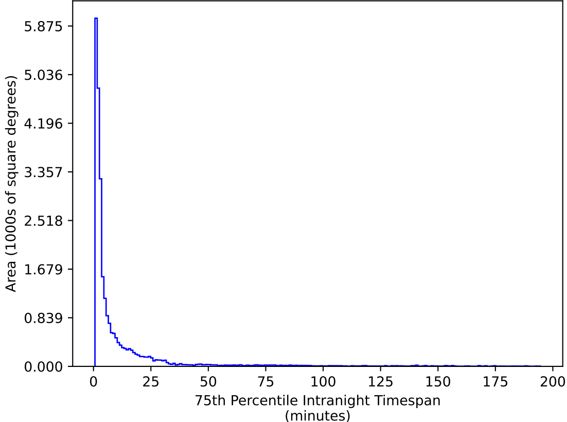
too_elab_r32_d2_giz_v3.4_10yrs All sky g band: 75th Percentile Intranight Timespan
