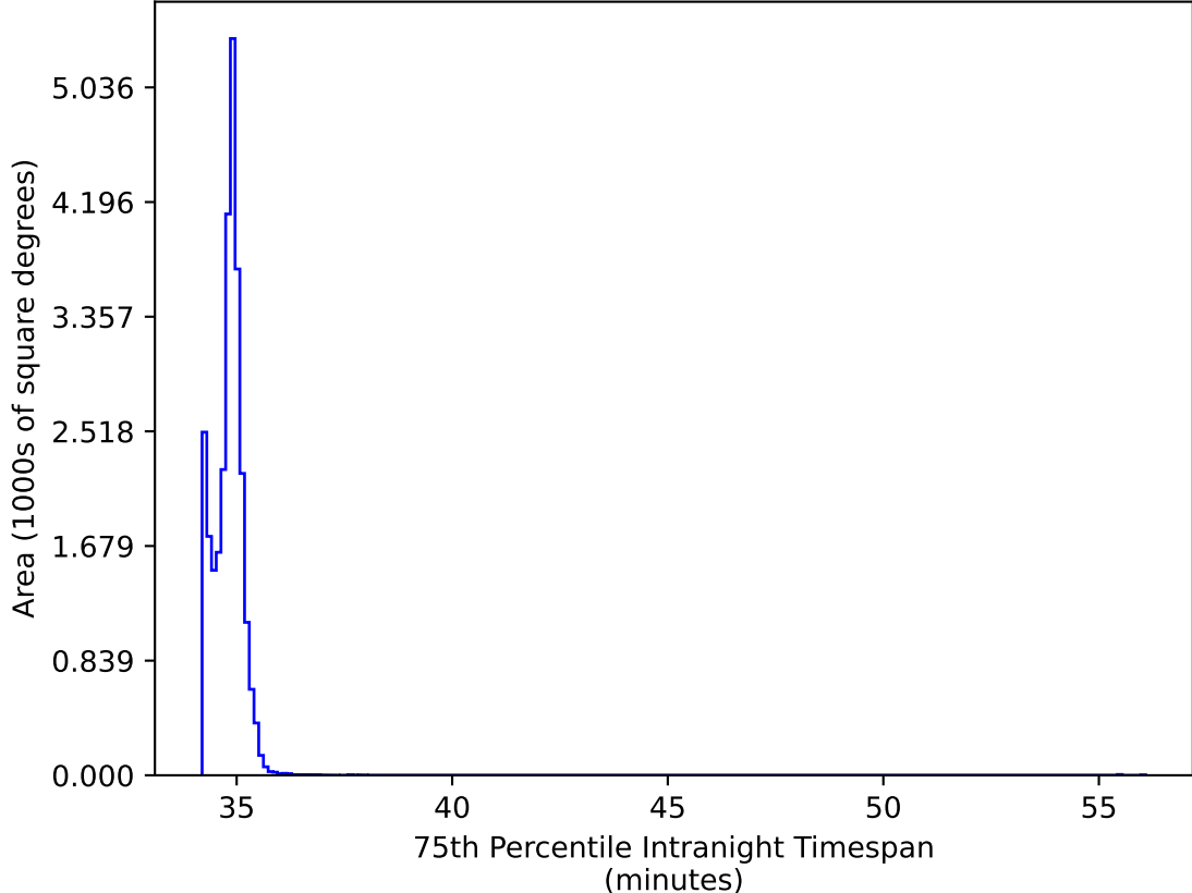
too_elab_r32_d2_giz_v3.4_10yrs All sky all bands: 75th Percentile Intranight Timespan
