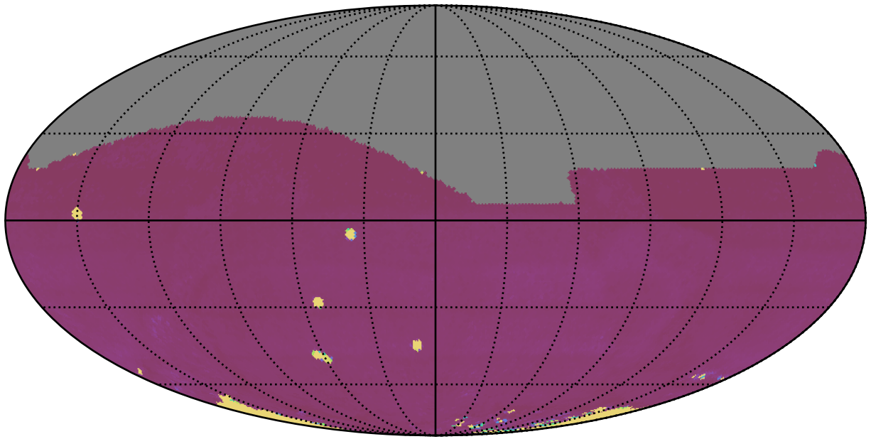
too_elab_r32_d2_giz_v3.4_10yrs All sky: 75th Percentile Intranight Timespan
