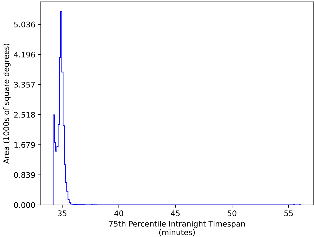
too_elab_r32_d2_giz_v3.4_10yrs All sky: 75th Percentile Intranight Timespan
