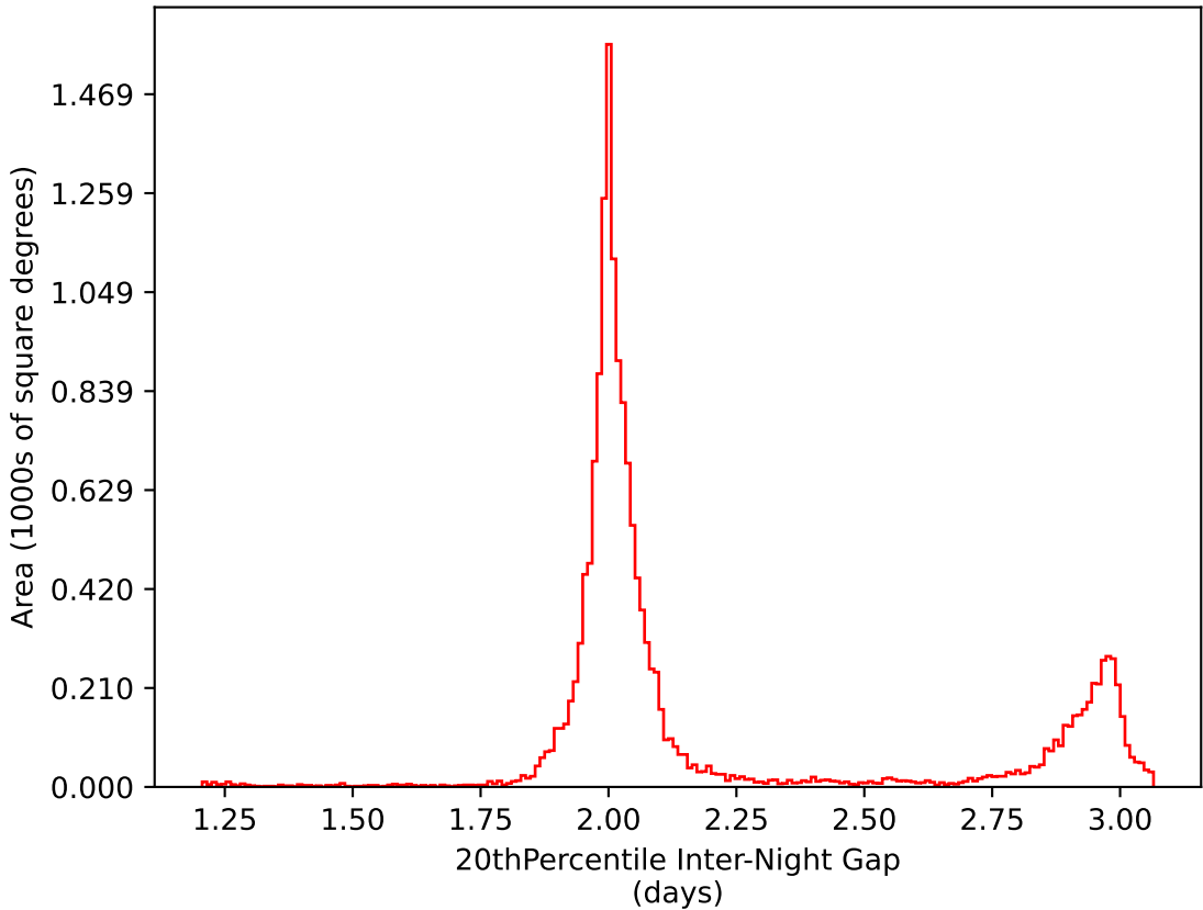
too_elab_r32_d2_giz_v3.4_10yrs WFD i band: 20thPercentile Inter-Night Gap
