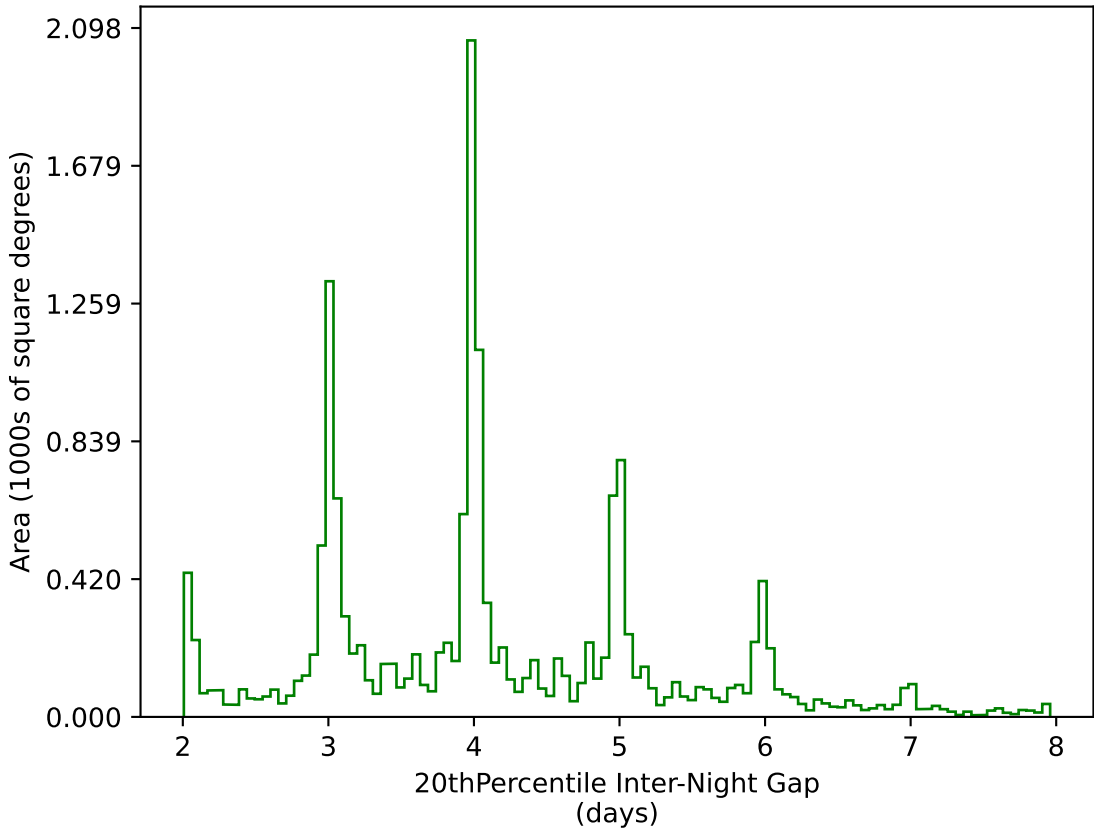
too_elab_r32_d2_giz_v3.4_10yrs WFD g band: 20thPercentile Inter-Night Gap
