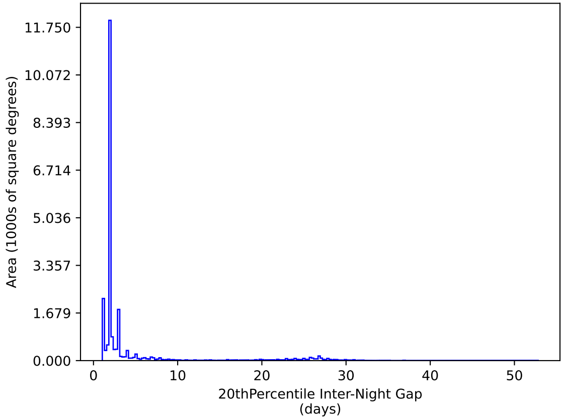
too_elab_r32_d2_giz_v3.4_10yrs All sky y band: 20thPercentile Inter-Night Gap
