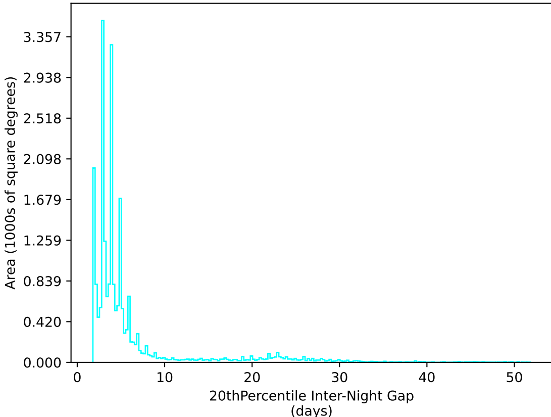
too_elab_r32_d2_giz_v3.4_10yrs All sky u band: 20thPercentile Inter-Night Gap
