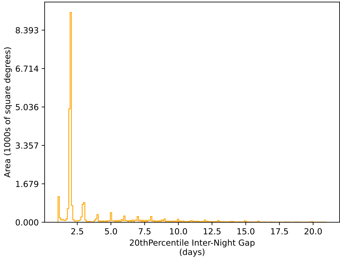
too_elab_r32_d2_giz_v3.4_10yrs All sky r band: 20thPercentile Inter-Night Gap
