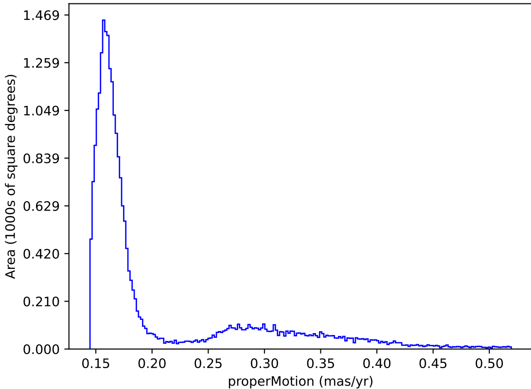
too_elab_r32_d2_giz_v3.4_10yrs : properMotion
