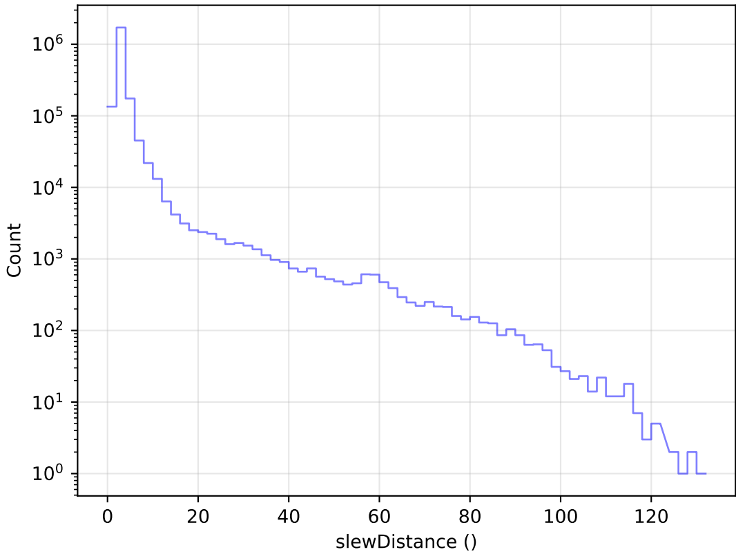
too_elab_r32_d2_giz_v3.4_10yrs All visits: Slew Distance Histogram
