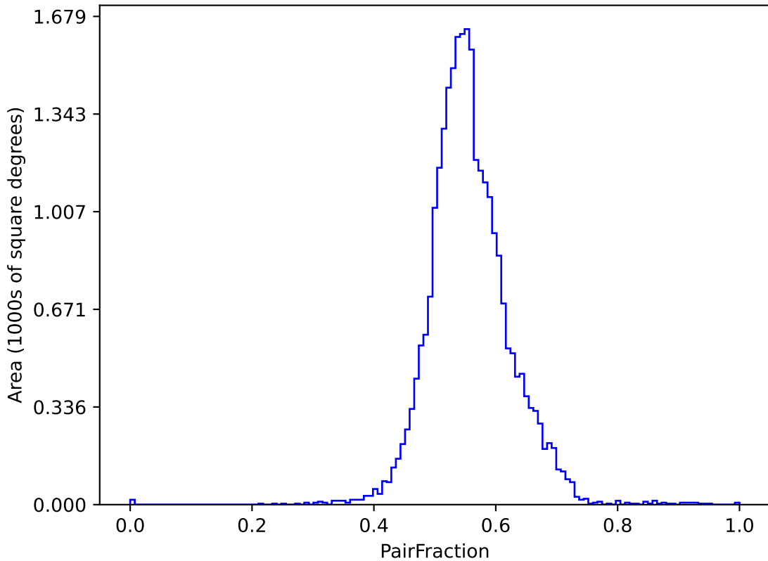
too_elab_r32_d2_giz_v3.4_10yrs (g or r or i): PairFraction
