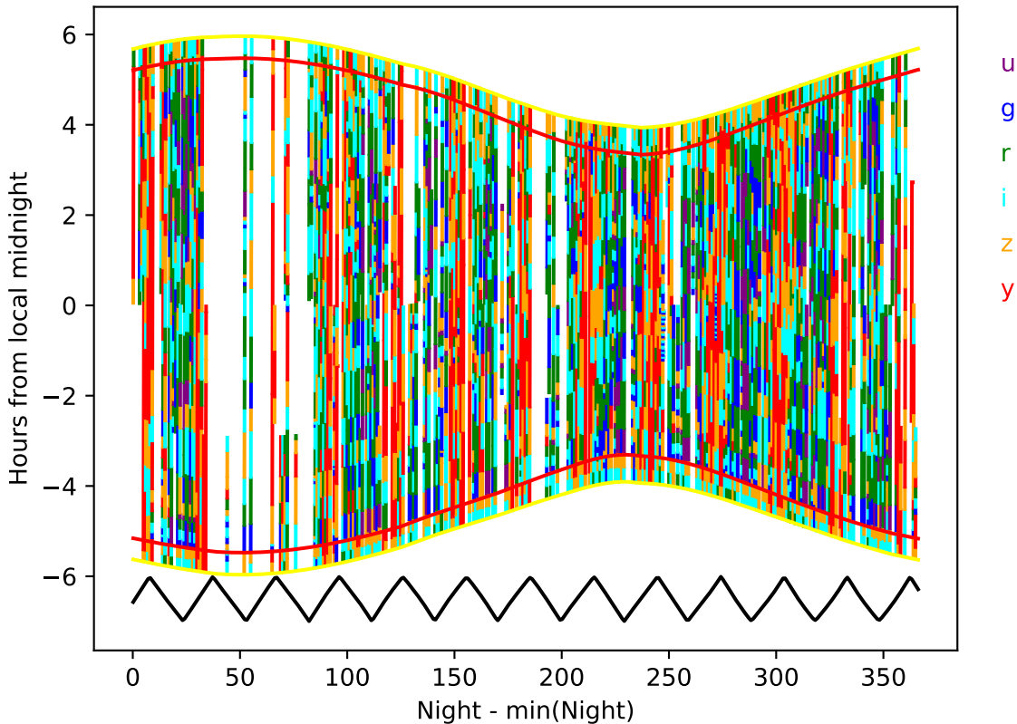
too_elab_r32_d2_giz_v3.4_10yrs year 3-4: Hourglass
