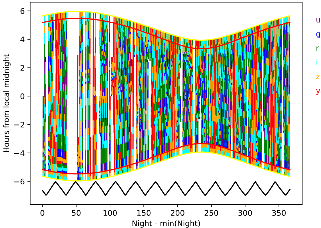
too_elab_r32_d2_giz_v3.4_10yrs year 2-3: Hourglass
