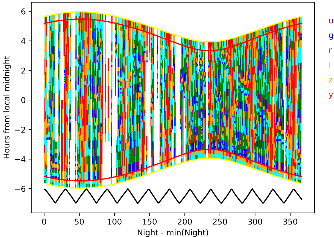
too_elab_r32_d2_giz_v3.4_10yrs year 1-2: Hourglass
