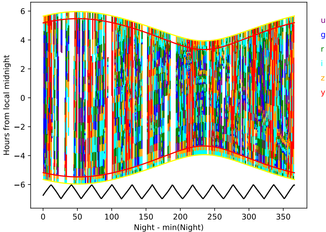
too_elab_r32_d2_giz_v3.4_10yrs year 0-1: Hourglass
