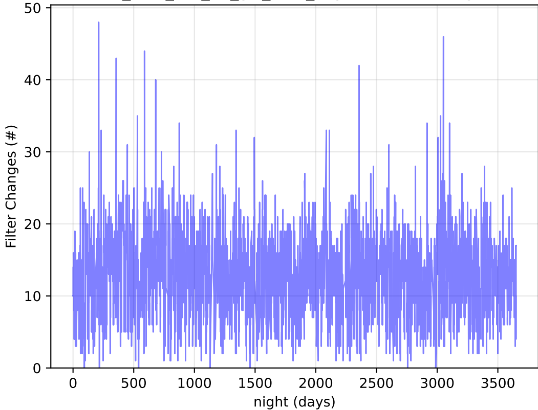
too_elab_r32_d2_giz_v3.4_10yrs : Filter Changes
