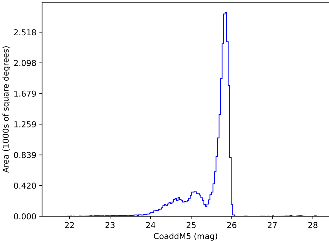
too_elab_r32_d2_giz_v3.4_10yrs z: CoaddM5
