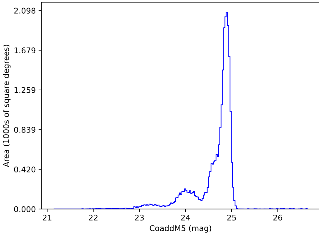
too_elab_r32_d2_giz_v3.4_10yrs y: CoaddM5
