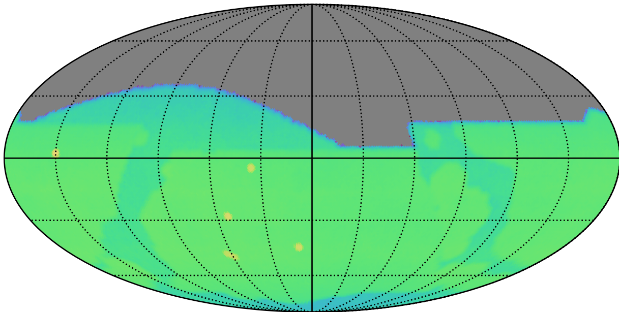
too_elab_r32_d2_giz_v3.4_10yrs : CoaddM5
