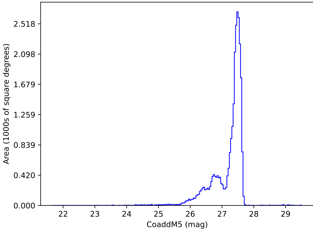
too_elab_r32_d2_giz_v3.4_10yrs : CoaddM5
