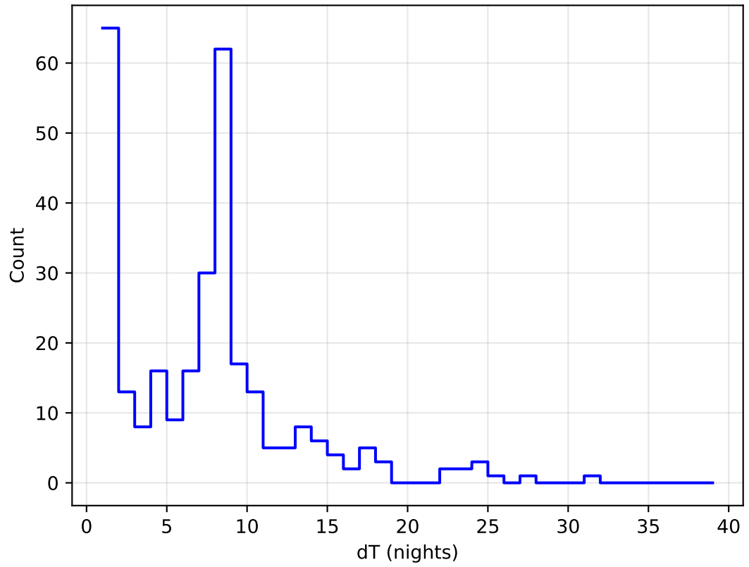
too_elab_r32_d2_giz_v3.4_10yrs all bands: DD:XMM_LSS Delta Nights Histogram
