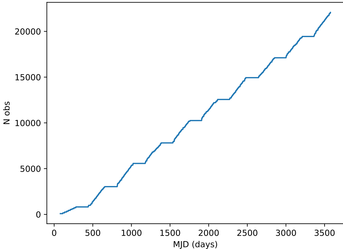
too_elab_r32_d2_giz_v3.4_10yrs all bands: DD:XMM_LSS Cumulative NVisits
