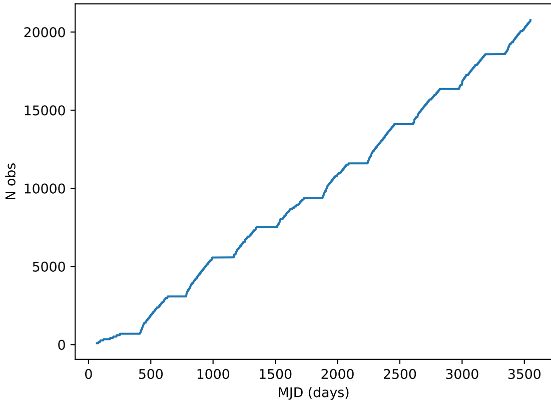
too_elab_r32_d2_giz_v3.4_10yrs all bands: DD:ELAISS1 Cumulative NVisits
