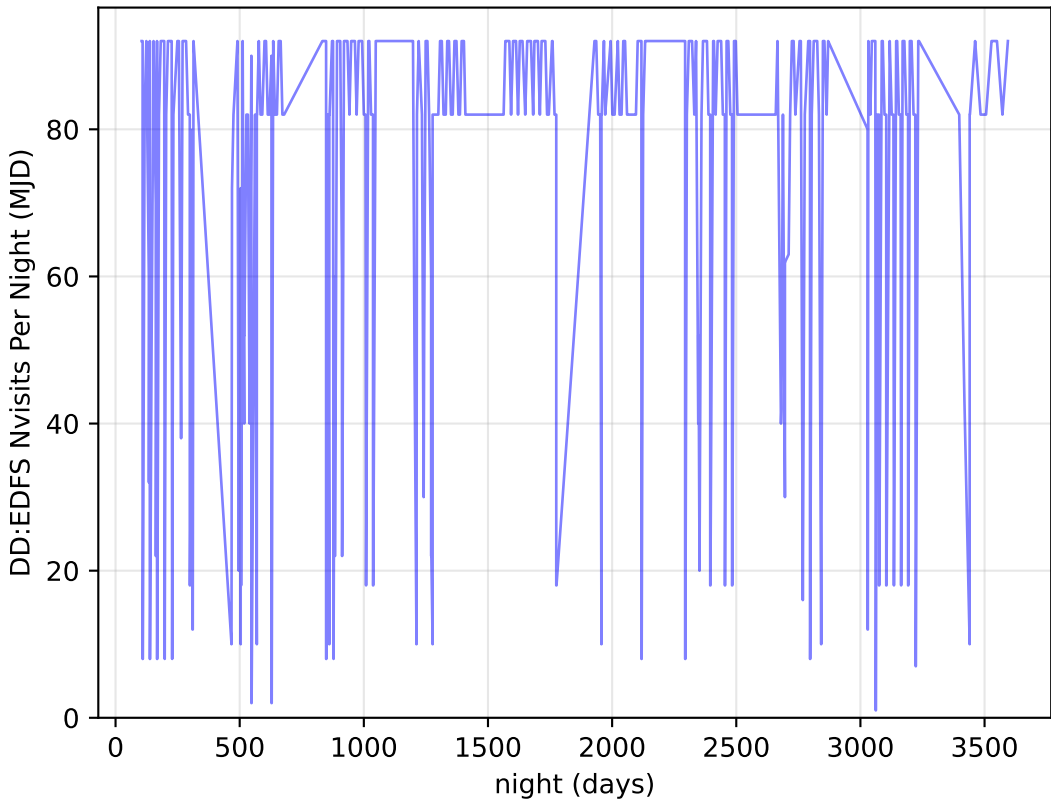
too_elab_r32_d2_giz_v3.4_10yrs all bands: DD:EDFS Nvisits Per Night
