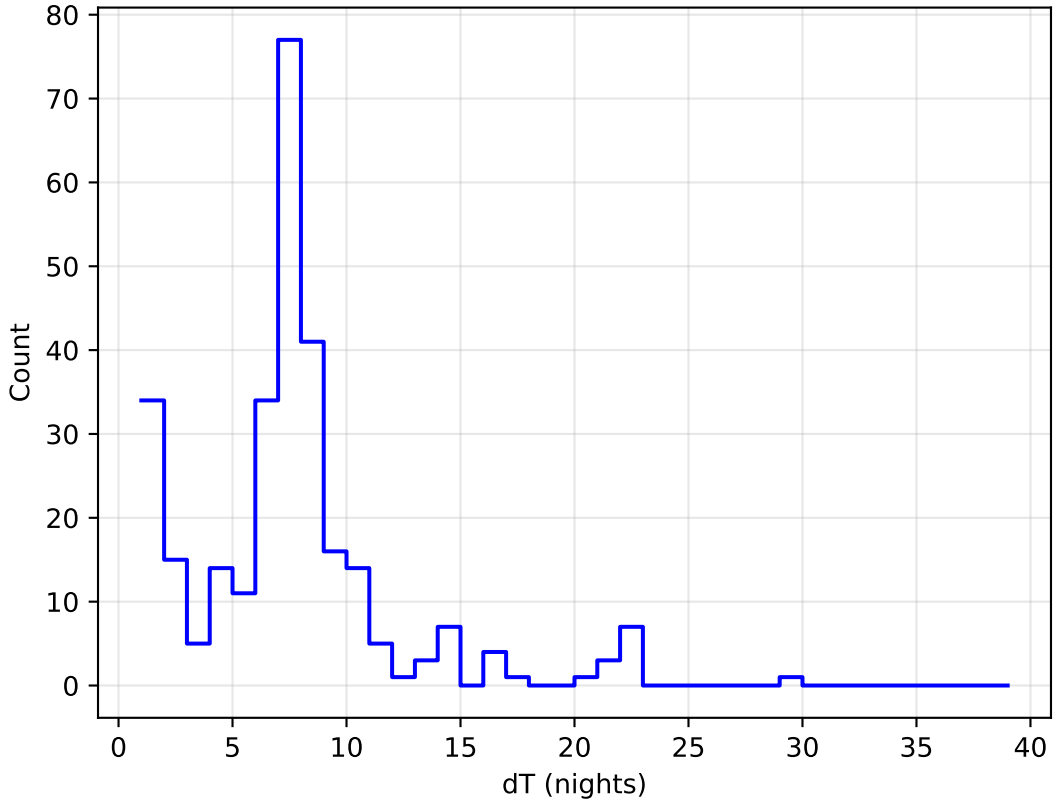
too_elab_r32_d2_giz_v3.4_10yrs all bands: DD:EDFS Delta Nights Histogram
