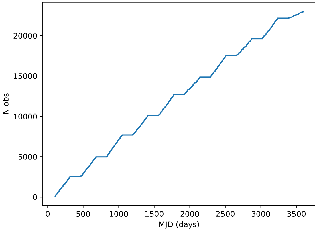
too_elab_r32_d2_giz_v3.4_10yrs all bands: DD:EDFS Cumulative NVisits
