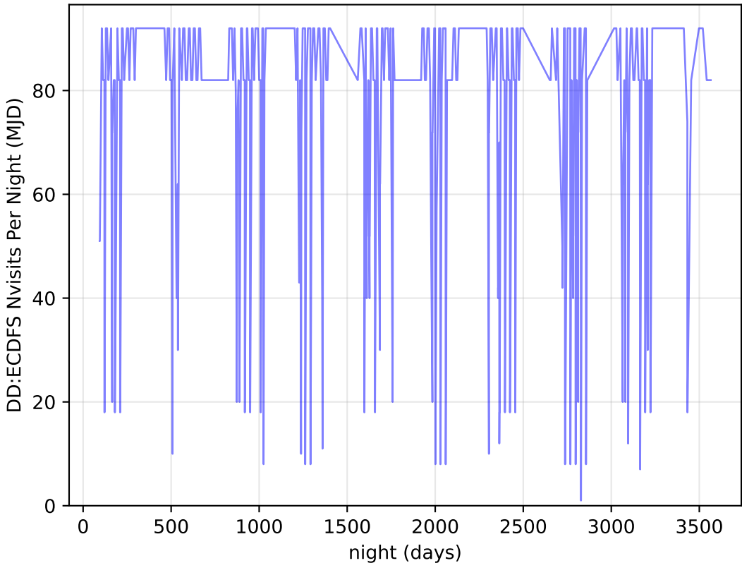
too_elab_r32_d2_giz_v3.4_10yrs all bands: DD:ECDFS Nvisits Per Night
