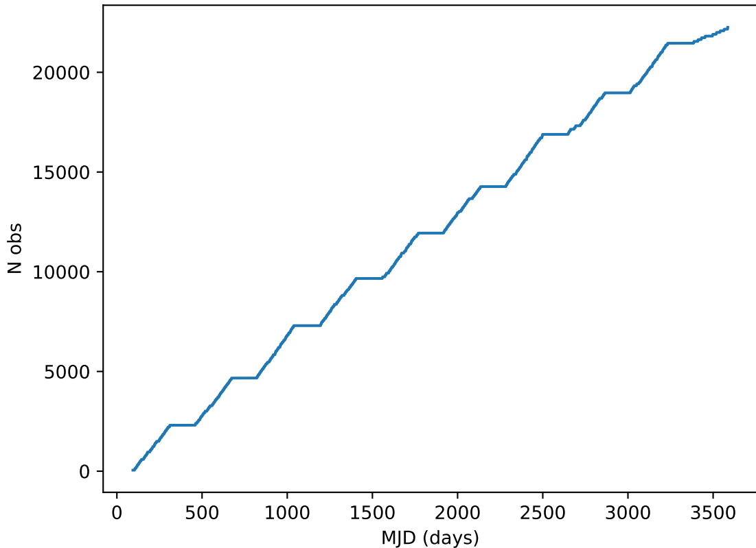
too_elab_r32_d2_giz_v3.4_10yrs all bands: DD:ECDFS Cumulative NVisits
