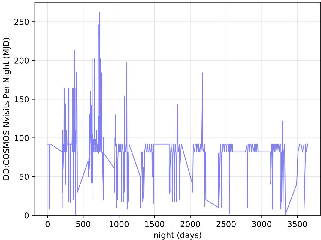
too_elab_r32_d2_giz_v3.4_10yrs all bands: DD: COSMOS Nvisits Per Night
