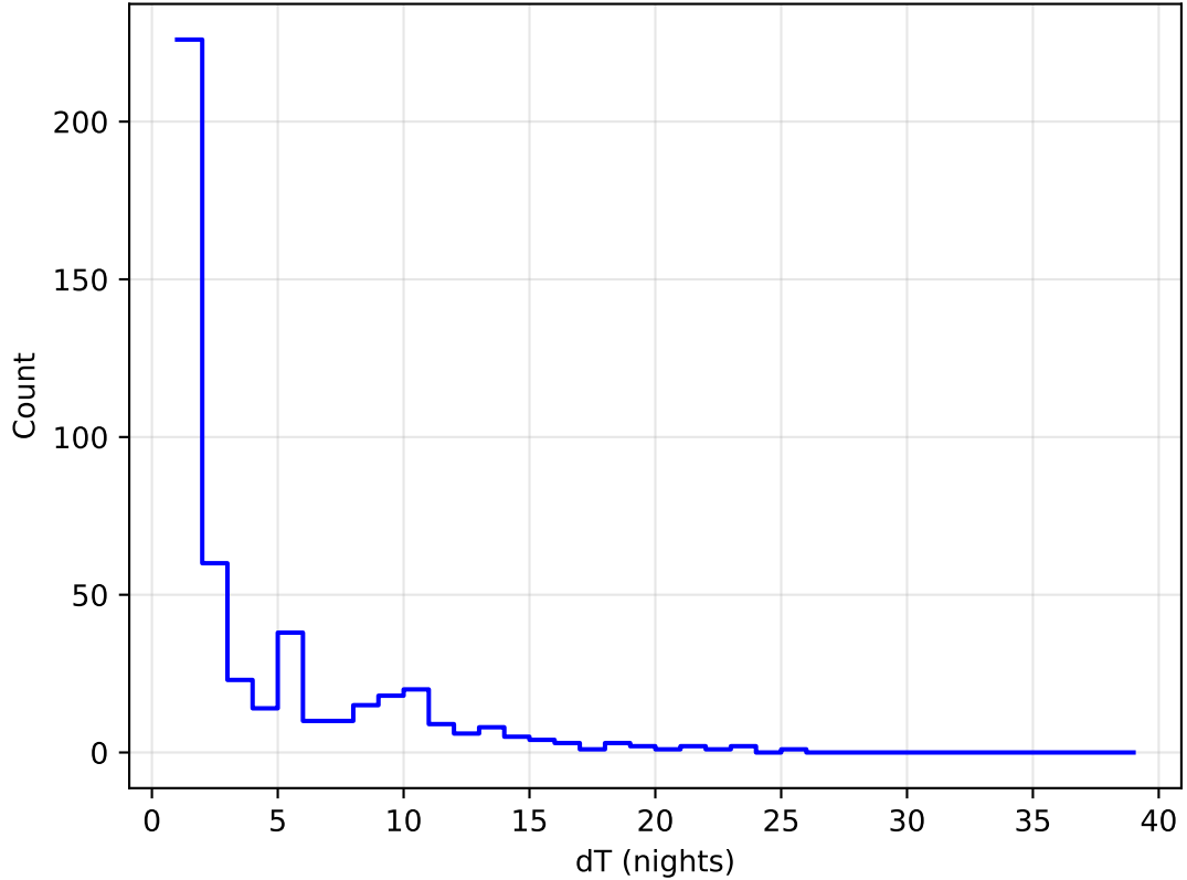
too_elab_r32_d2_giz_v3.4_10yrs all bands: DD: COSMOS Delta Nights Histogram
