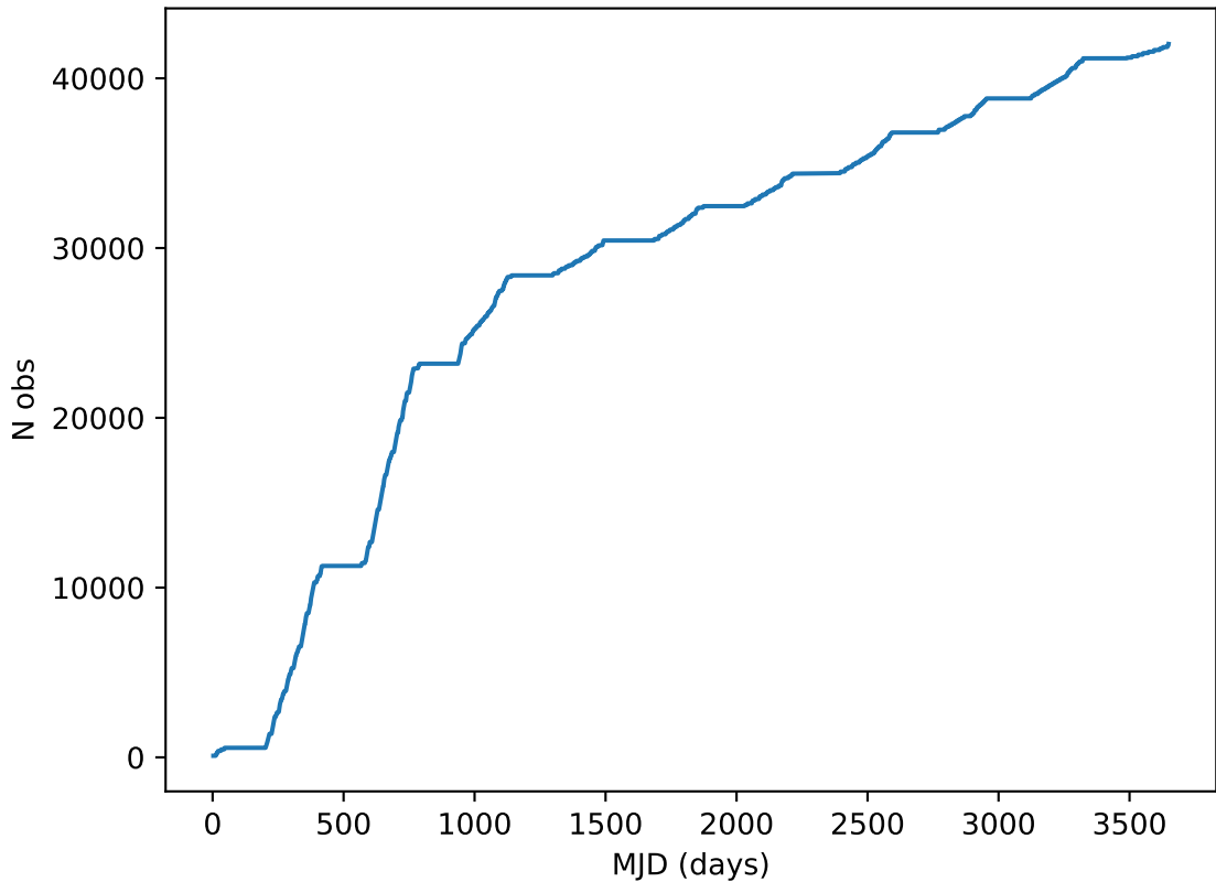
too_elab_r32_d2_giz_v3.4_10yrs all bands: DD:COSMOS Cumulative NVisits
