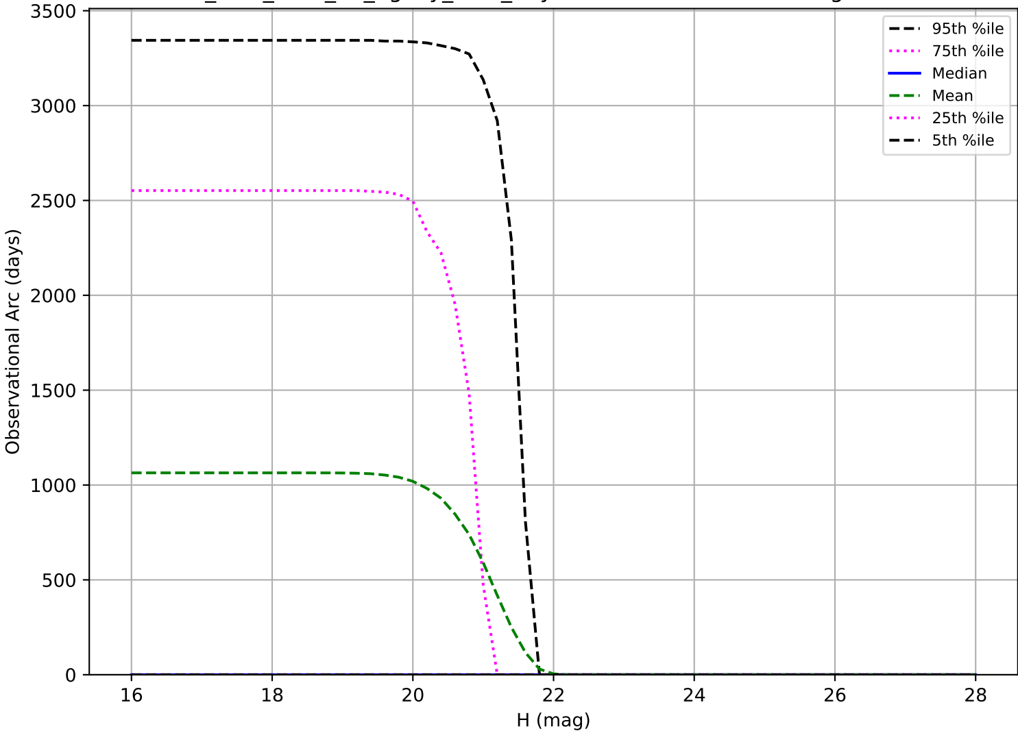
too_elab_r256_d3_ugrizy_v3.4_10yrs: Observational Arc Length Vatira
