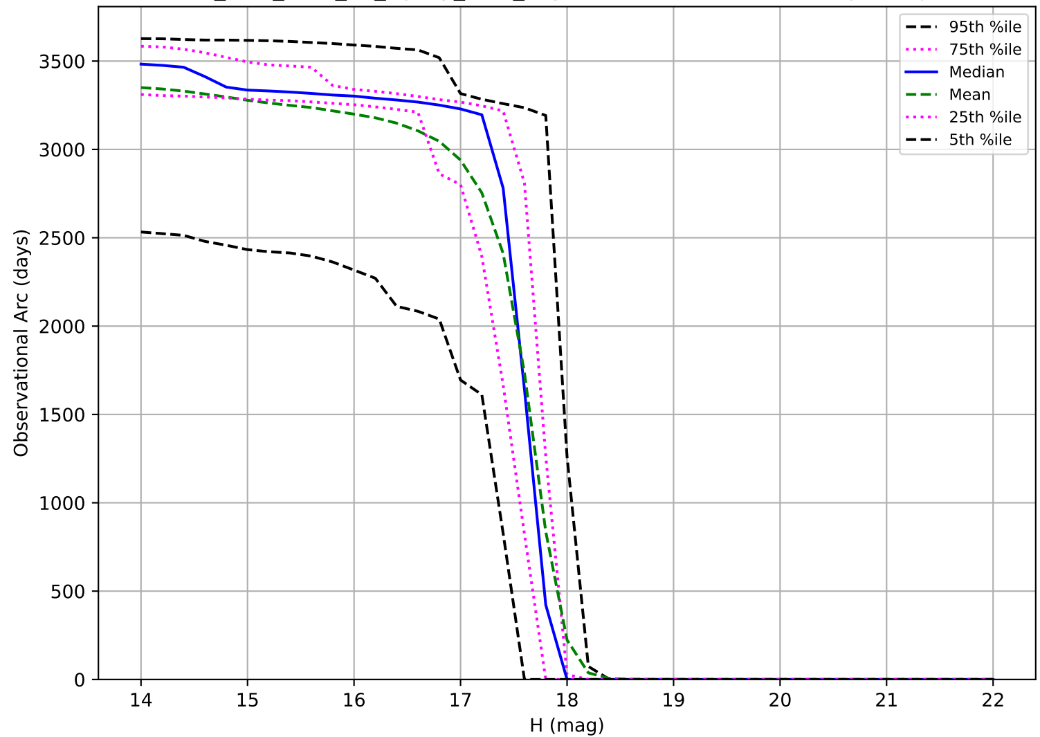
too_elab_r256_d3_ugrizy_v3.4_10yrs: Observational Arc Length Trojan
