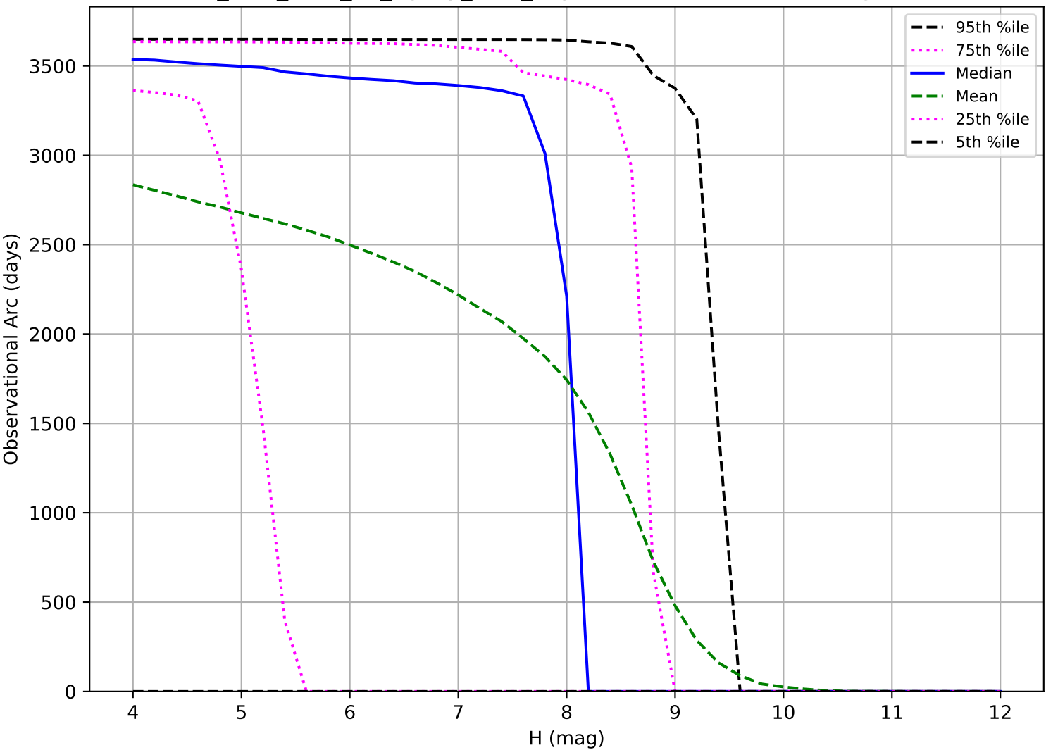
too_elab_r256_d3_ugrizy_v3.4_10yrs: Observational Arc Length TNO
