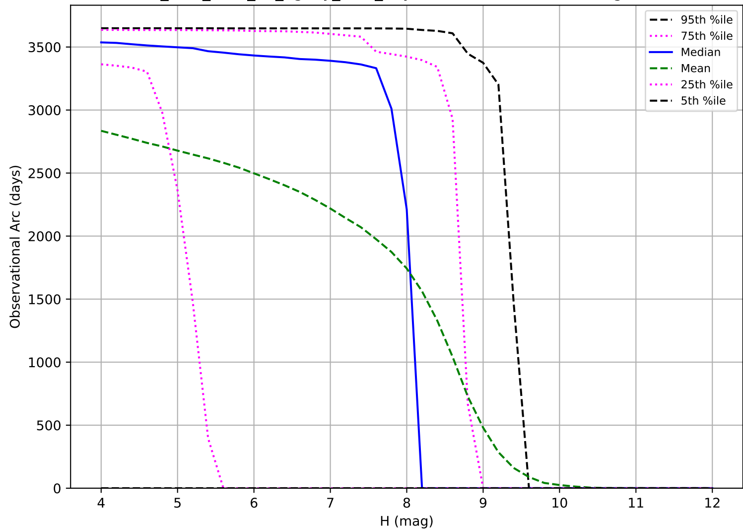
too_elab_r256_d3_ugrizy_v3.4_10yrs: Observational Arc Length TNO
