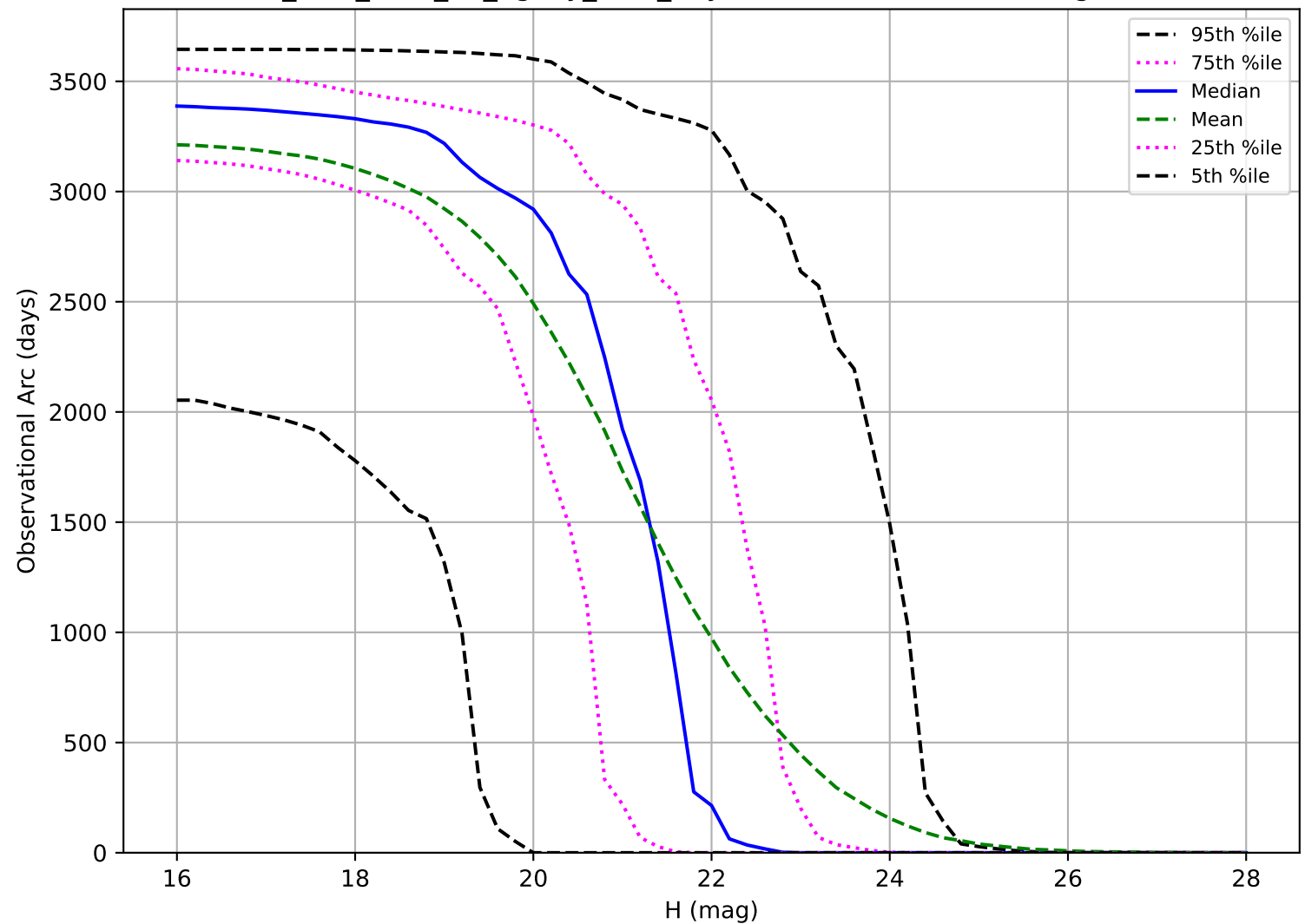
too_elab_r256_d3_ugrizy_v3.4_10yrs: Observational Arc Length PHA
