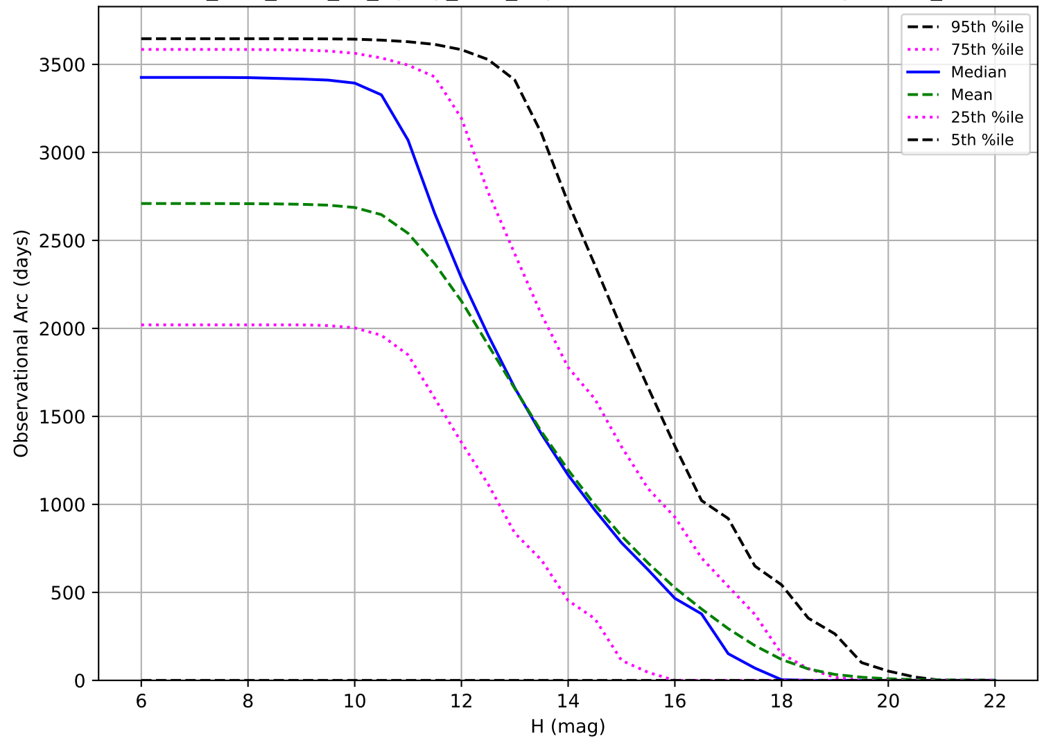
too_elab_r256_d3_ugrizy_v3.4_10yrs: Observational Arc Length OCC_r5
