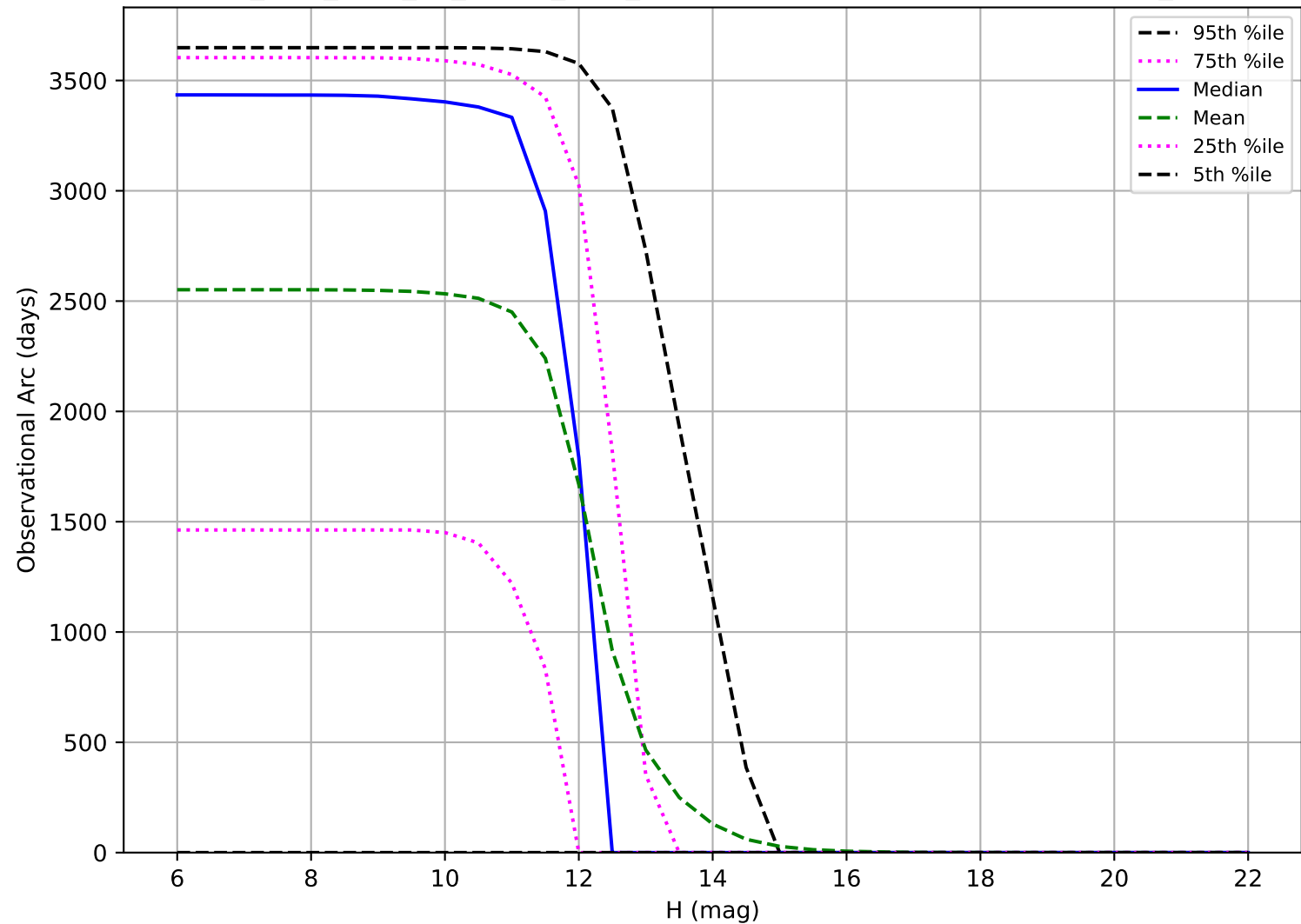
too_elab_r256_d3_ugrizy_v3.4_10yrs: Observational Arc Length OCC_r20
