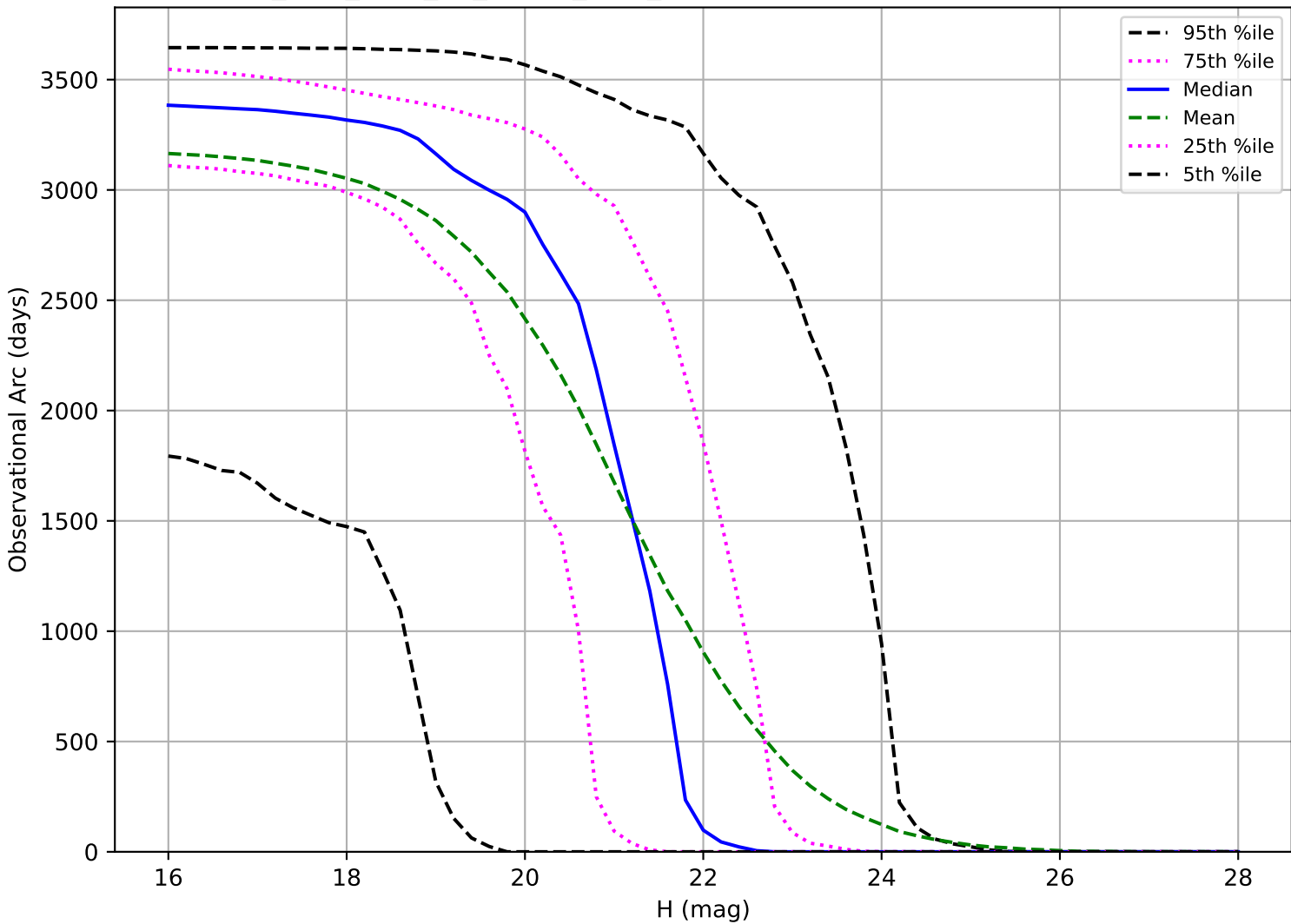
too_elab_r256_d3_ugrizy_v3.4_10yrs: Observational Arc Length NEO
